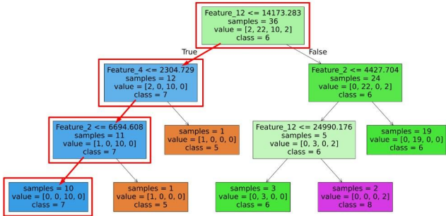
MsPacman PPO Decision Tree
